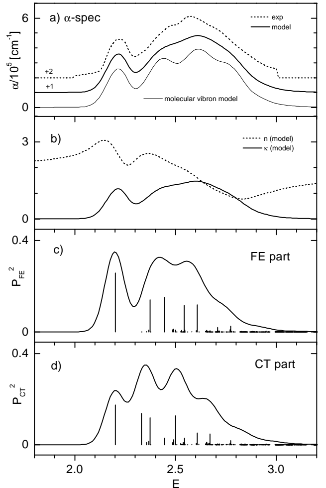
FIG. 9: Experimental low temperature absorption spectra of PTCDA and model fit. Panel a shows the comparison for the absorption coefficient \alpha . The model fit (parameters see text) is done with a large phonon basis (as in Fig. 7) but a comparison with the molecular vibron model for the same parameters is also given. Panel b shows the optical constants n , \kappa corresponding to the model fit. Panel c shows the actual eigenstates and the Frenkel part of their spectral weight. In panel d, the CT part of the spectral weight is given. The stick spectra are broadened by Gaussians with a constant width \sigma = 48 meV corresponding to the width of the lowest state in the fit.
