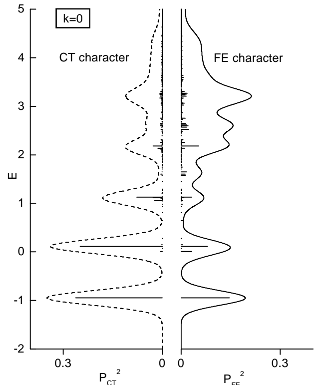
FIG. 7: Eigenstates of the extended Holstein model for Frenkel-CT mixing (47) at total momentum k = 0 . Parameters: J = 0.5 , g = 1 , D = 0 , t_e = t_h = 0.5 , g_e = g_h = 1/\sqrt{2} . The Frenkel parameters and the illustration correspond to Fig. 1. P_{\text{FE}}^2 shows the spectral weights (Frenkel character) of the Frenkel-part, P_{\text{CT}}^2 shows the spectral weights of the symmetric CT part. The broadened spectra are both normalized to an area of 0.5.
