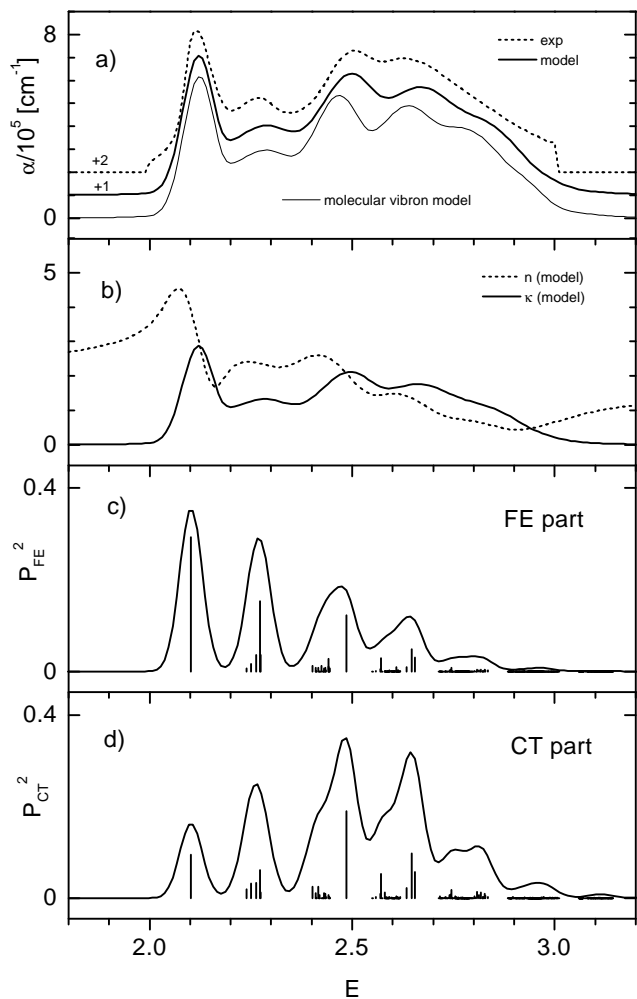
FIG. 10: Experimental absorption spectra of MePTCDI and model fit. Panel a shows the comparison for the p -polarized \alpha spectra, the parameters are given in the text. The model spectrum is shown for a large phonon cloud basis (as in Fig. 7) and the molecular vibron model. Panel b gives the optical constants from the model. Panels c and d show the actual eigenstates and their composition as explained in Fig. 9. The broadening in c and d is constant \sigma = 28 meV as for the lowest peak in the experimental spectrum. Due to the variable broadening in the fit, the second large peak at \approx 2.3 eV from panel c appears in the \alpha and \kappa spectra of panels a and b only as a broad feature with lower peak value.
