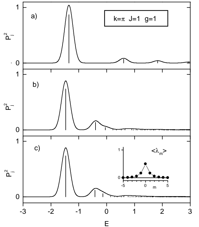
FIG. 6: Convergence of absorption spectra at the bottom of the band for J = 1 and g = 1 . Panels a, b and c show the results for the same basis sets as in Fig. 3. The area of the broadened spectra is normalized to 0.45.
