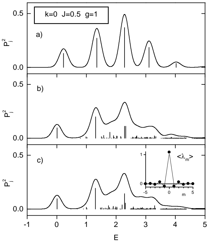
FIG. 3: Convergence of absorption spectra at the top of the band for J = 0.5 and g = 1 (intermediate coupling, rather small J ). Panel a shows the results for the molecular vibron model (26). Panels b and c show spectra for a large phonon cloud basis. Going from b to c, the maximum cloud radius M is increased from 5 to 6 and on each relative site m the maximum occupation number \nu_m is increased by one. This increases the number of symmetric basis states from 1587 in panel b to 4485 in c. The sticks always show the spectral weight according to Eq. (17). The solid lines are convolutions of the stick spectra with a Gaussian as in Fig. 1 (normalized to area 0.5). The shape of the thus broadened spectrum in panel c has almost converged, particularly for energies E < 2.5 . The inset in panel c shows the displacement cloud of the lowest state as in Fig. 1.
