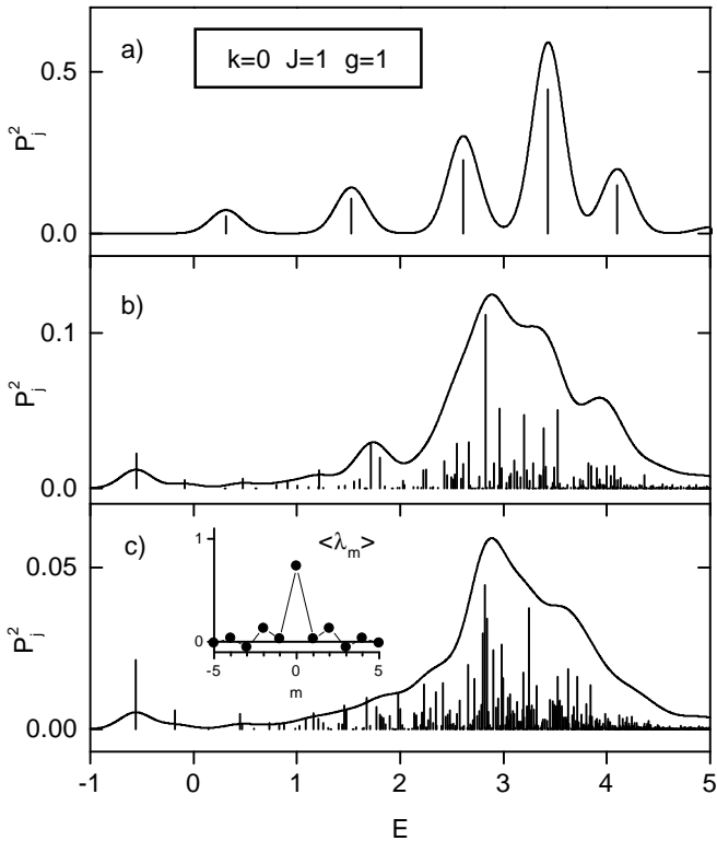
FIG. 5: Convergence of absorption spectra at the top of the band for J = 1 and g = 1 . Panels a, b and c show the results for the same basis sets as in Fig. 3. With increasing number of states, the spectral weight of the individual states in the higher energy region decreases. Therefore, the y-axis scaling and the normalization of the broadened spectra is different in each panel. (Area = 0.5 in panel a, area = 0.3 in panel b and area = 0.09 in panel c.)
