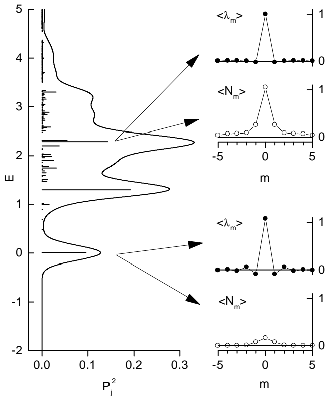
FIG. 1: Illustration of the eigenstates and their properties for a numerical solution of the Holstein model (1) with parameters J = 0.5 and g = 1 at total momentum k = 0 . In the left panel, the optically active eigenstates are shown at a vertical energy axis. The sticks indicate the spectral weight P_j^2 of each state according to Eq. (17). For a visualization of the resulting spectrum, the stick spectrum is convolved with a Gaussian (standard derivation \sigma = 0.15 ) and the broadened spectrum is scaled for easy superposition (here: area \int f(E)dE = 0.5 ). In the right panels, the occupation number clouds \langle \hat{N}_m \rangle and displacement clouds \langle \hat{\lambda}_m \rangle are shown for two particular eigenstates (cf. comments to Eqs. (20) and (21)).
