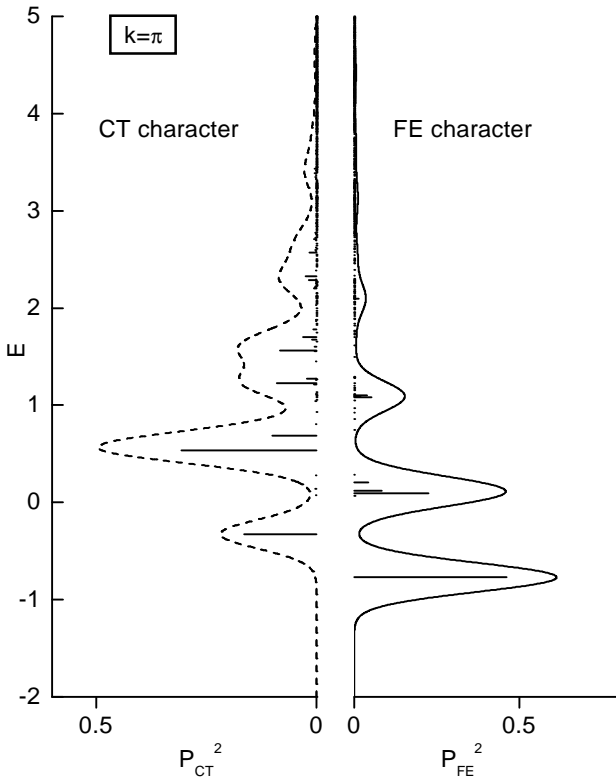
FIG. 8: Eigenstates of the extended Holstein model for Frenkel-CT mixing (47) at total momentum k = \pi . Parameters as in Fig. 8. Because of t_e = t_h , the electronic FE and CT states do not mix and all eigenstates have either pure FE or pure CT character.
