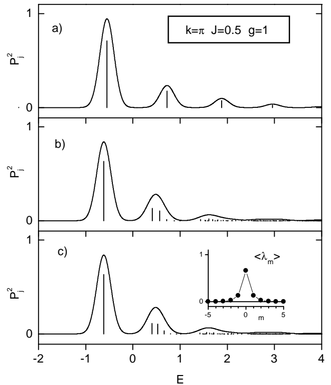
FIG. 4: Convergence of absorption spectra at the bottom of the band for J = 0.5 and g = 1 . Panels a, b and c show the results for the same basis sets as in Fig. 3. The broadened spectra are again normalized to area = 0.5.
