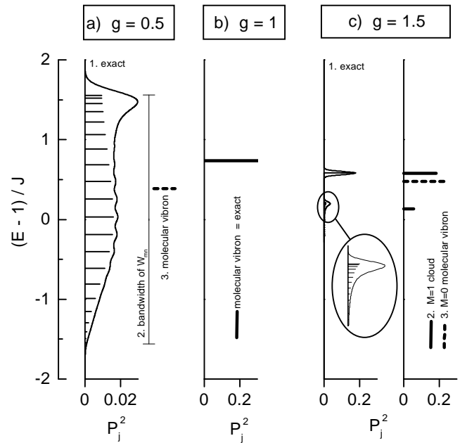
FIG. 2: Perturbative treatment J \rightarrow 0 of the one-phonon subspace for three coupling parameters g . The “exact” stick spectra are numerical solutions of the one-phonon Hamiltonian (33) for a phonon-cloud radius of M = 20 . The envelopes are convolutions of the stick spectra with Gaussians of appropriate width. Fig. 2a represents the small- g case, where a broad one-phonon sideband is formed. The “exact” solution in graph 1 is compared to the bandwidth of the free-phonon part ( W_{mn} from Eq. (37)) in graph 2 and to the position of the single active state from the molecular vibron model (26) in graph 3. Fig. 2b represents the g = 1 case, where the molecular vibron model becomes exact. Fig. 2c represents the large- g case, in which the exciton interacts mainly with a nearest neighbor phonon cloud. The “exact” numerical solution in graph 1 resembles the approximate solution (39) for a nearest neighbor cloud ( M = 1 ) in graph 2. The single state from the molecular vibron model ( M = 0 ) is shown in graph 3.
