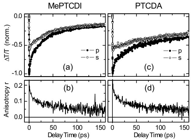
FIG. 4: Polarization dependent ps-pump-probe measurements and the resulting anisotropies for MePTCDI ((a),(b)) and PTCDA ((c),(d)). p and s denote parallel and perpendicular polarization of pump and probe beam, respectively.
